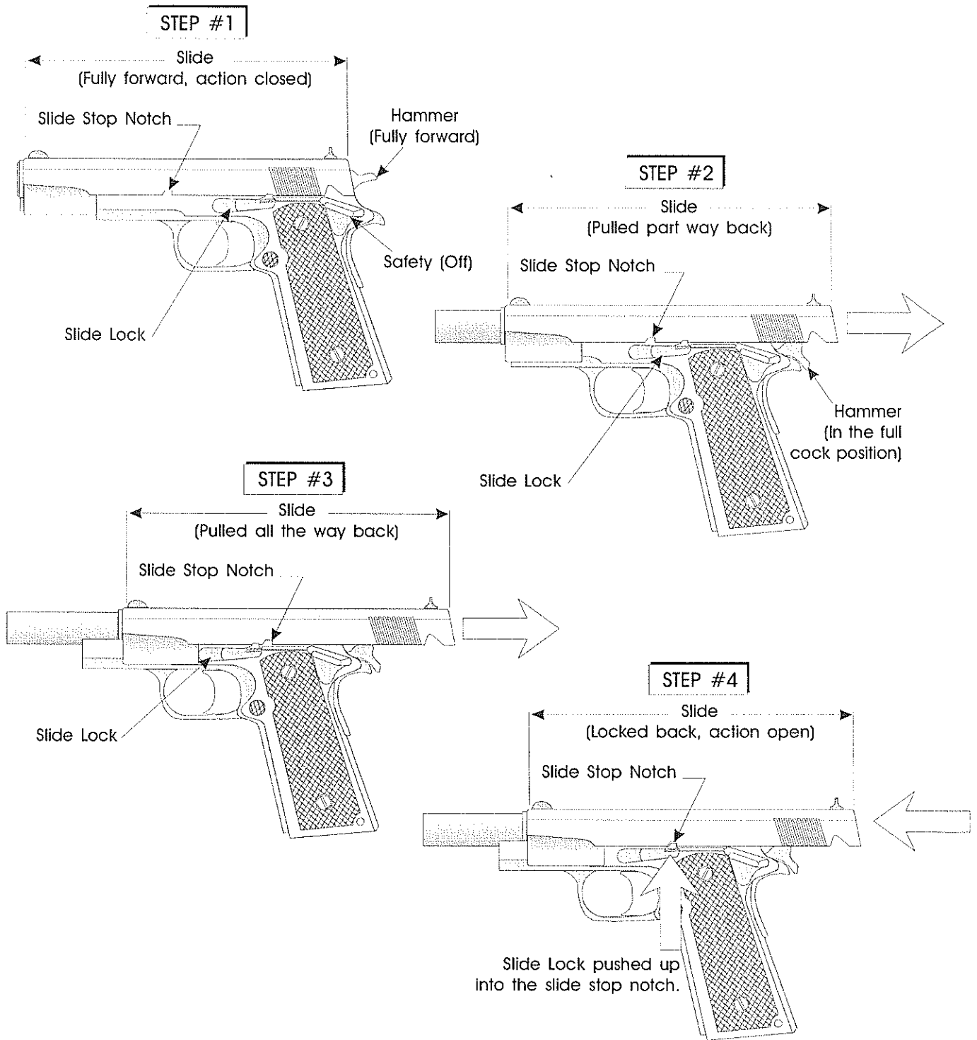
Figure 4-14 Locking the slide to the rear
