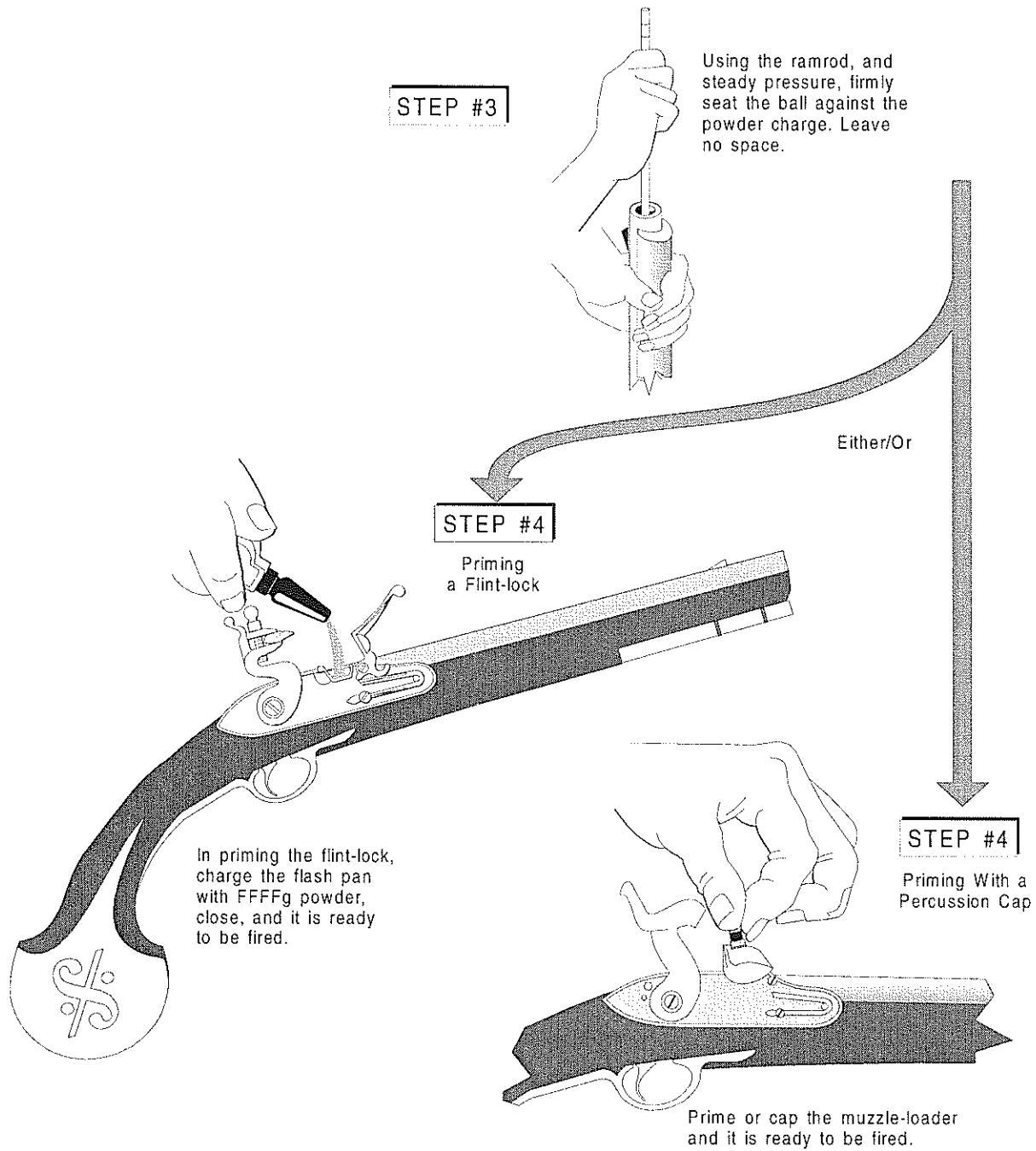
Figure 4-3 (continued) Loading a muzzle-loader
