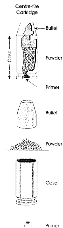
Figure 3-8 Centre-fire bullet, powder charge, case, and primer
