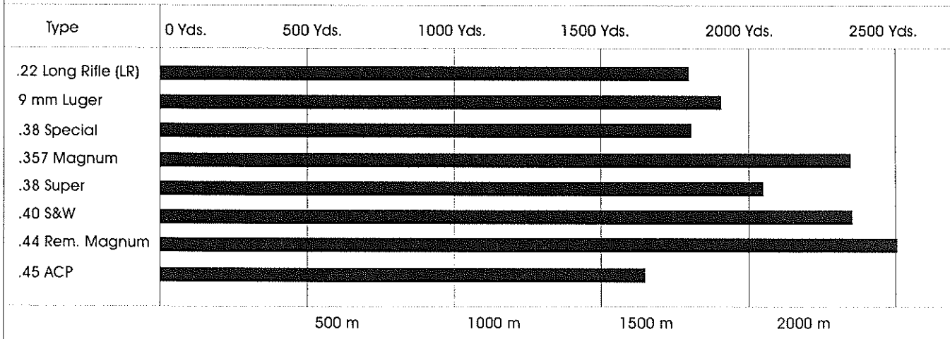
Dangerous Range of Handgun Ammunition
