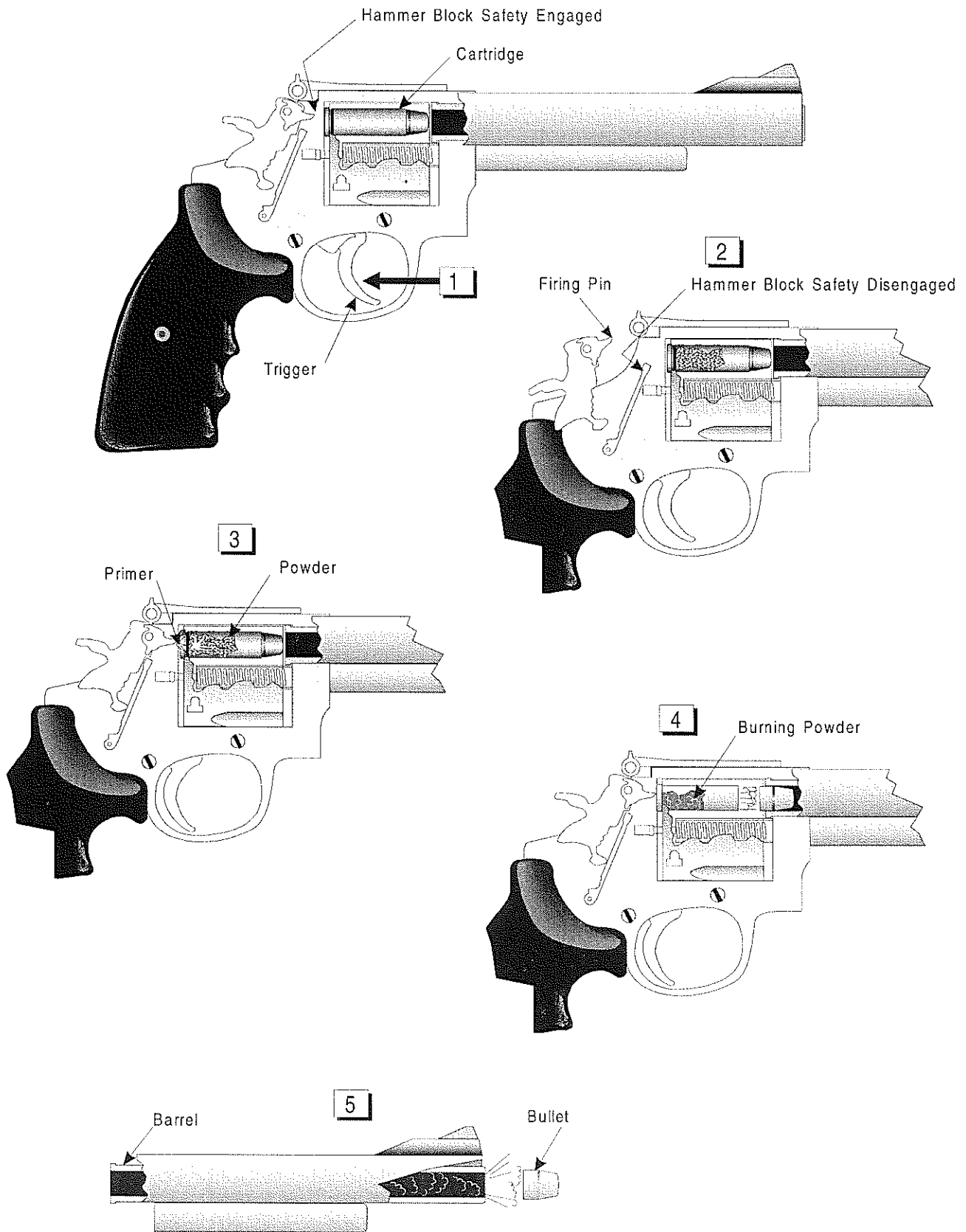
Figure 1-9 Firing sequence
